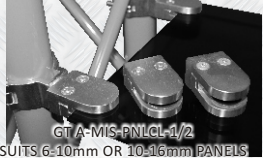
GT A-MIS-PNLCL-1/2 SUITS 6-10mm OR 10-16mm PANELS
